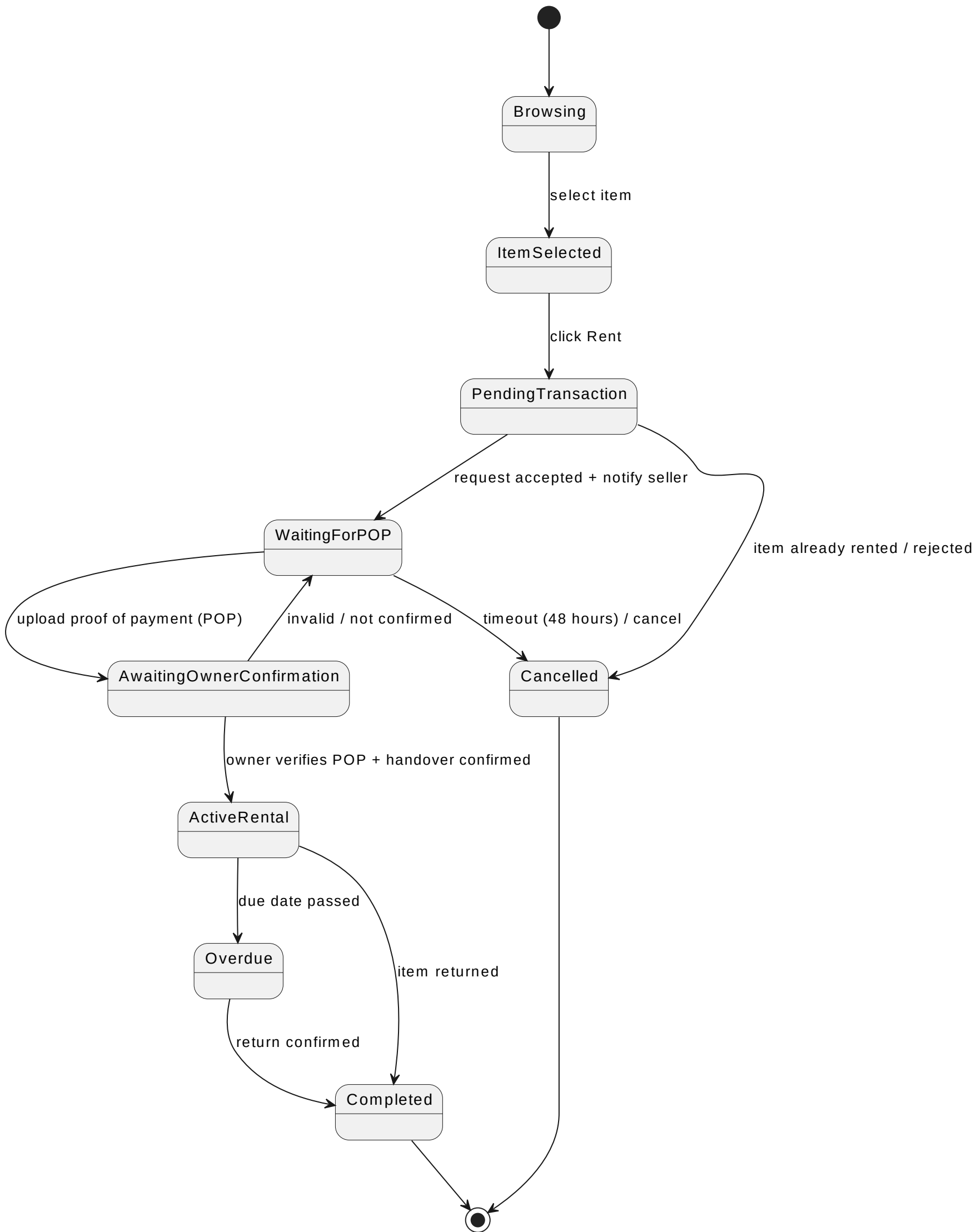
State Machine Diagram - Request to Rent Item
